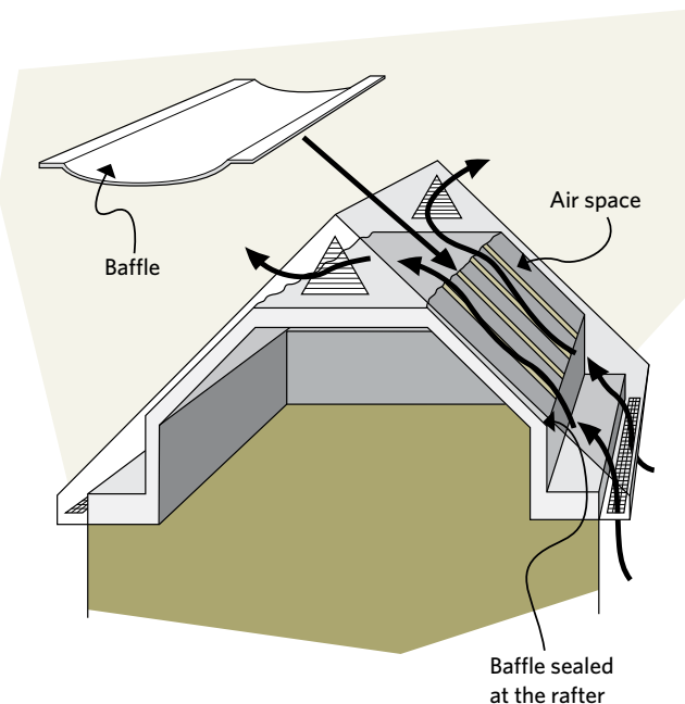
Figure 5-19 Ventilation occurs between sections through attic rafter vents installed in the rafter section
