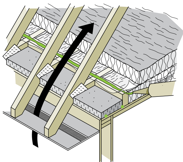
Figure 5-9 Installation of polyethylene sheets over attic joists
