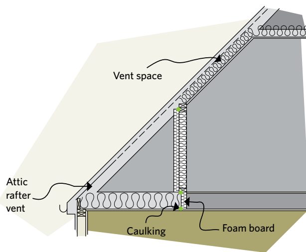
Figure 5-17 Rigid insulation can be nailed over the studs of the knee-wall section
