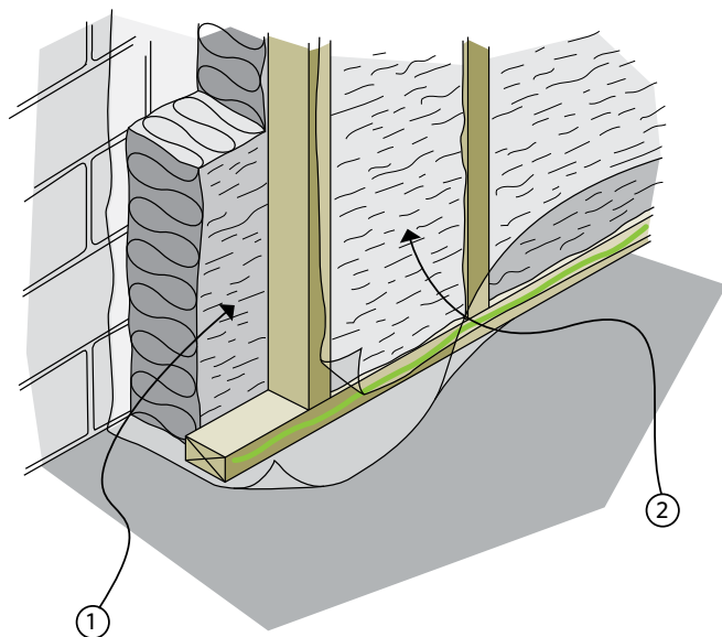
Figure 6-14 Double layer batt insulation in a framed wall
