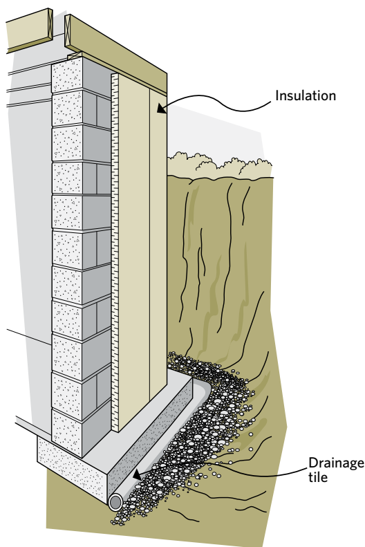
Figure 6-5 Draining-type insulations must be installed vertically all the way down to the footings
