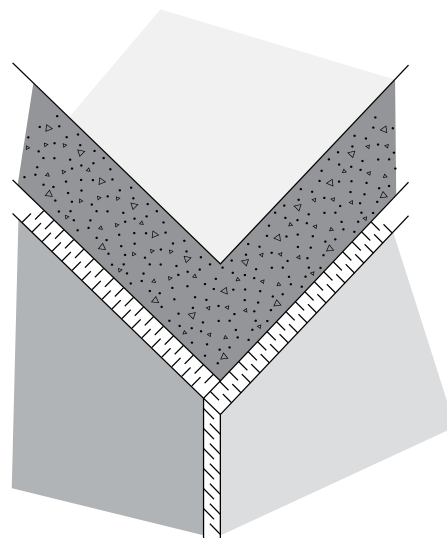
Figure 6-6 The insulation should overlap at corners
