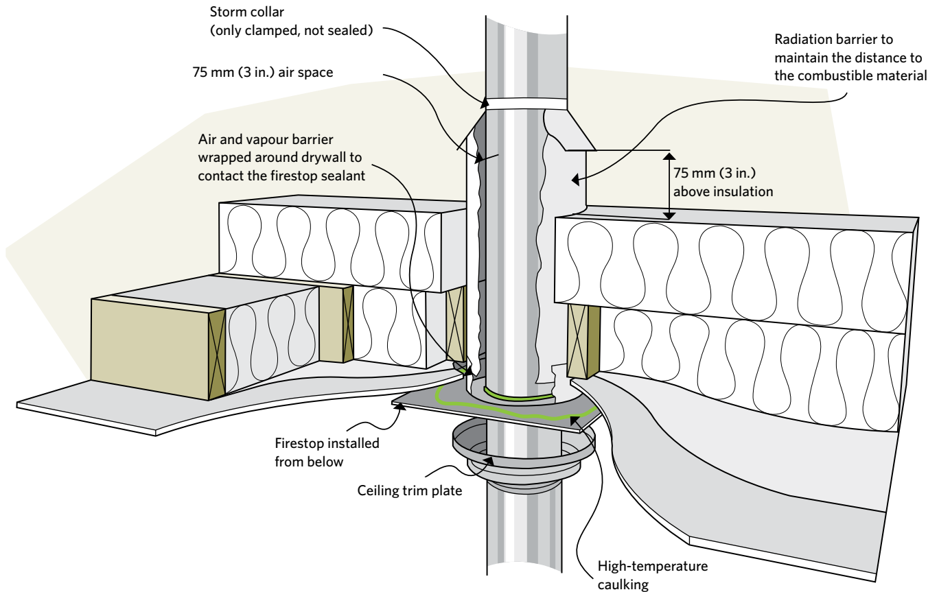
Figure 5-4 Keep combustibles away from a metal chimney
