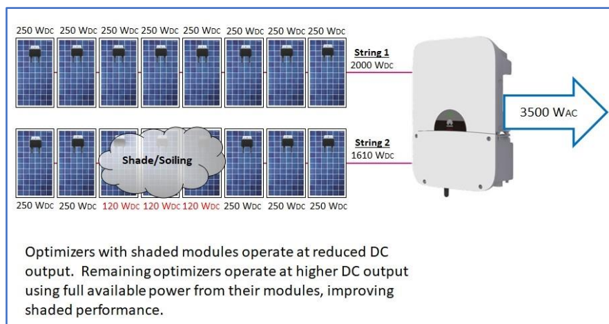
Figure 32: Optimized String Inverter - Shaded Operation - courtesy of Riverside Energy Systems with product image courtesy of Huawei
