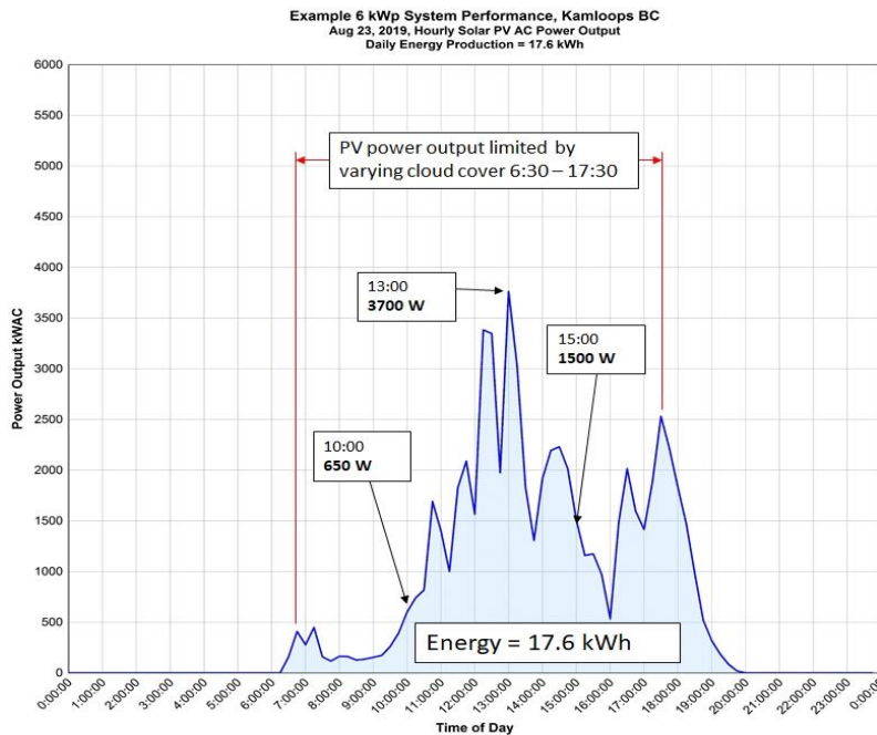
Figure 37: 6 kWp PV System Output Power, Aug 23, 2019 - courtesy Riverside Energy Systems
