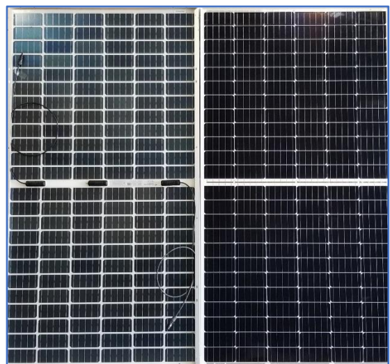
Figure 29: Two Bi-facial Solar Modules- back surface shown on left, front surface shown on right - courtesy of Riverside Energy Systems
