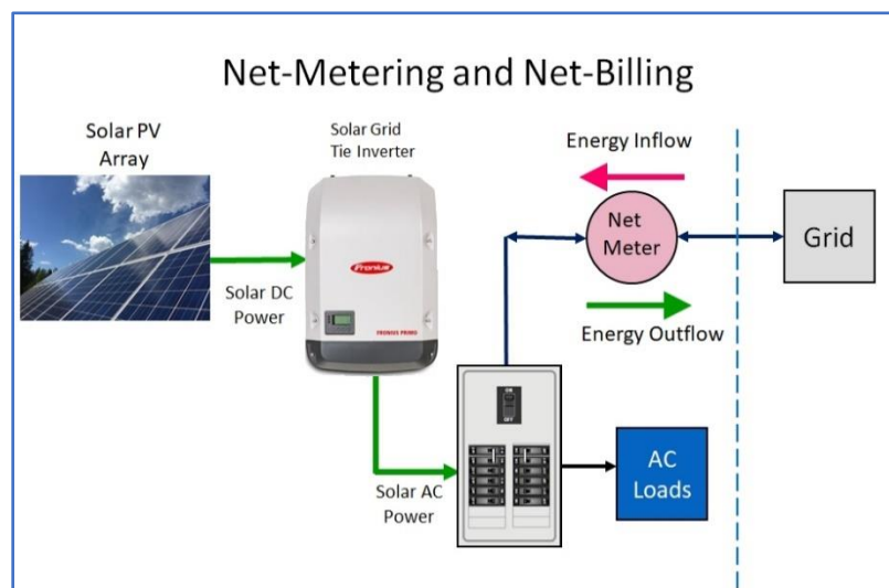
Figure 5: Electrical Configuration for Net-Metering and Net-Billing - courtesy of Riverside Energy Systems with Inverter image courtesy of Fronius
