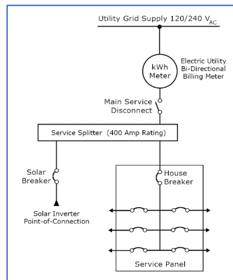
Figure 21: Service Splitter used as Point-of-Connection
