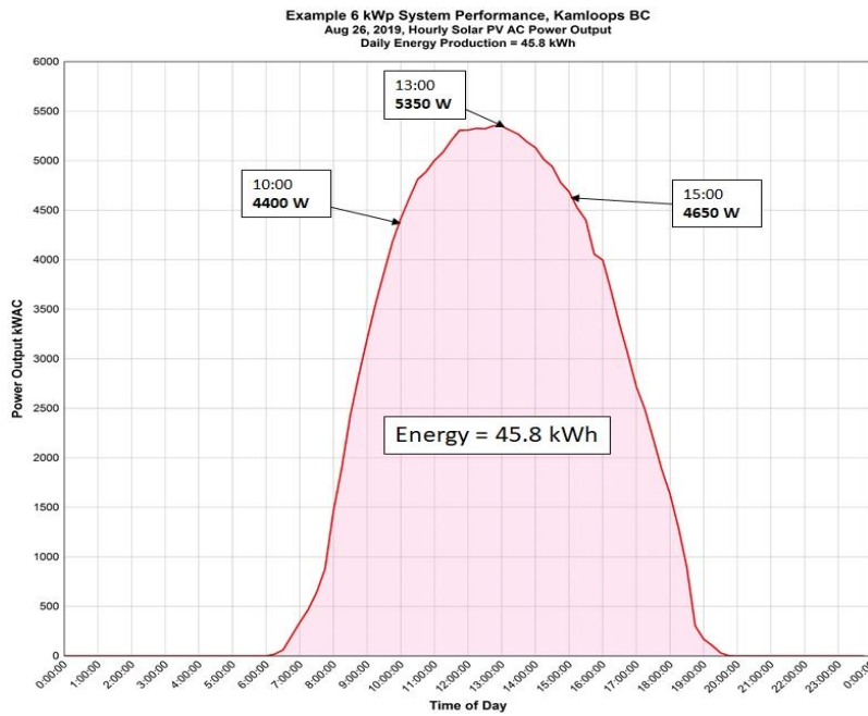
Figure 36: 6 kWp PV System AC Output Power, Aug 26, 2019 - courtesy Riverside Energy Systems
