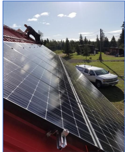
Figure 24: Racking Attachment to Standing Seam Metal Roofing - courtesy Riverside Energy Systems
