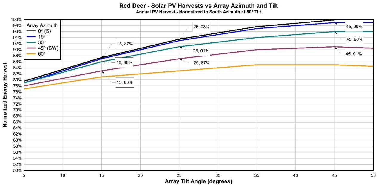
Figure 40: Red Deer AB, Effects of Azimuth and Tilt on Annual Solar PV Energy Production - courtesy Riverside Energy Systems
