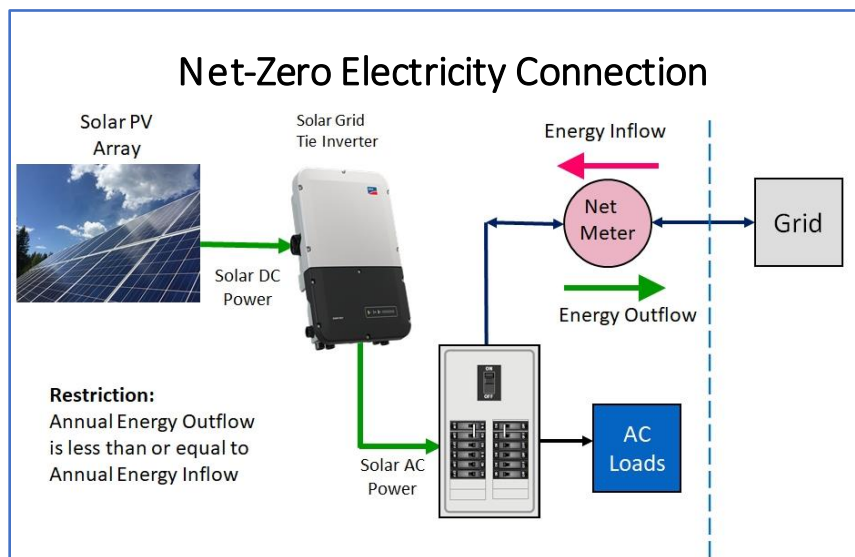
Figure 7: Electrical Configuration for Net-Zero Electricity Connections - courtesy of Riverside Energy Systems with Inverter image courtesy of SMA
