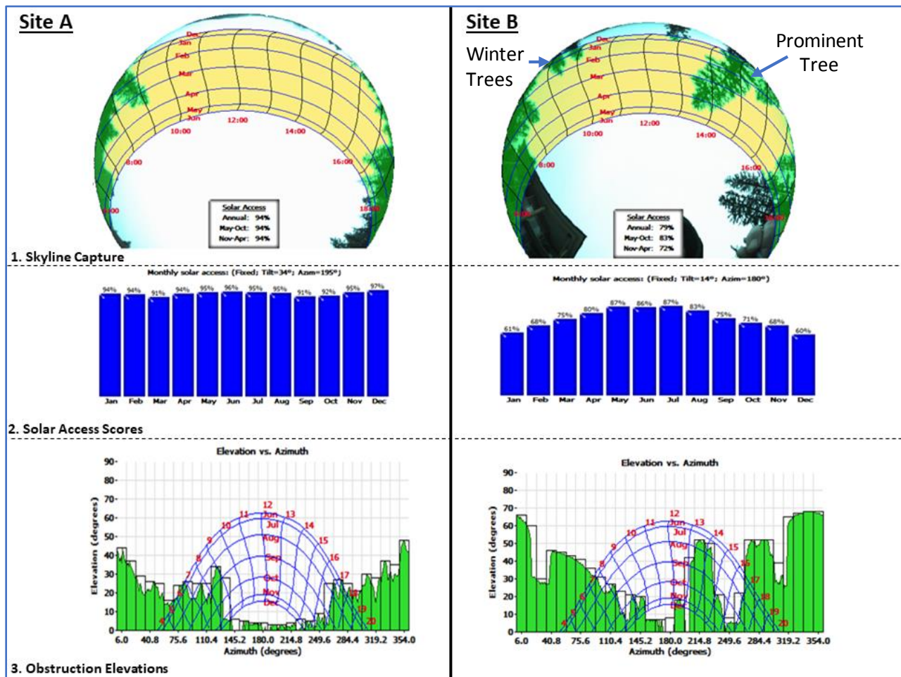
Figure 38: Solar Access and Shading Analysis - Contrasting Two Sites - courtesy of Riverside Energy Systems
