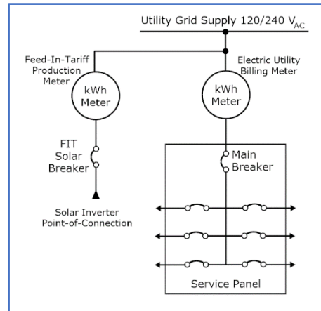
Figure 18: Feed-in-Tariff Point-of-Connection
