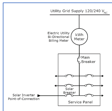
Figure 19: Main service panel Point-of-Connection
