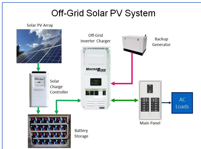
Figure 9: Electrical Configuration for an Off-Grid Solar PV System - courtesy of Riverside Energy Systems with product images courtesy of Magnum-Sensata
