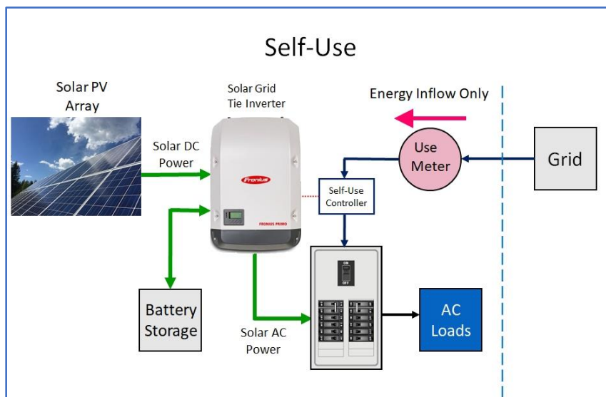
Figure 8: Electrical Configuration for Self-Use - courtesy of Riverside Energy Systems with Inverter image courtesy of Fronius
