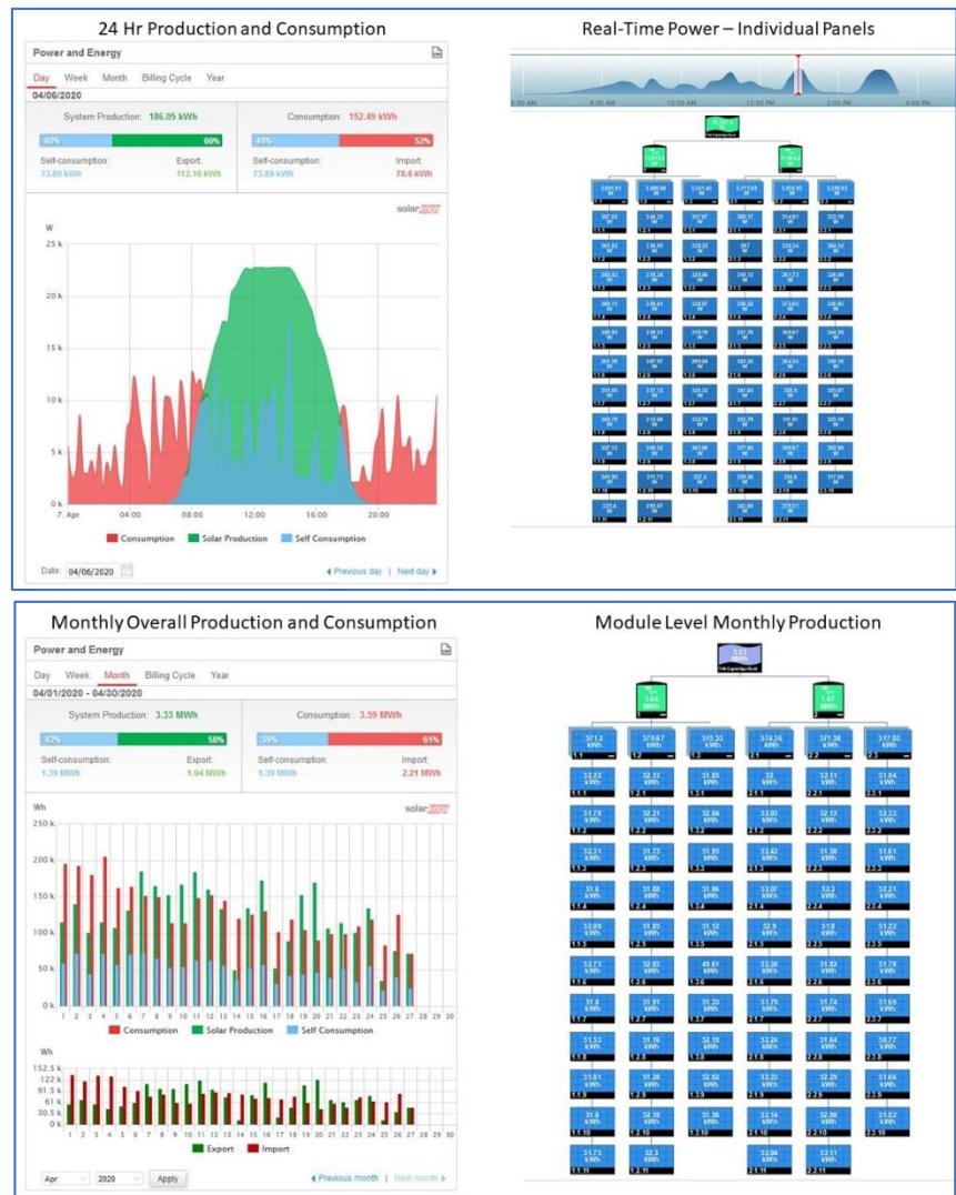
Figure 35: Example of an advanced energy display showing solar energy production and energy consumption for daily and monthly time periods - courtesy of Riverside Energy Systems
