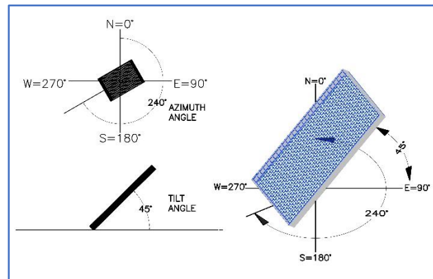
Figure 39: Solar PV Array Orientations - Azimuth and Tilt Angle - courtesy of Riverside Energy Systems
