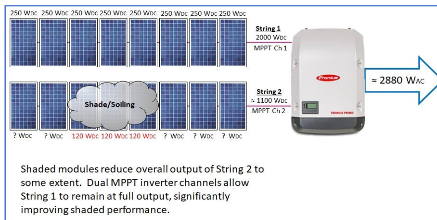
Figure 31: String Inverter with Dual MPPT Channels - Shaded Operation - courtesy of Riverside Energy Systems with inverter image courtesy of Fronius Canada
