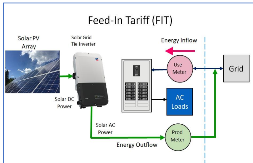
Figure 4: Electrical Configuration for Feed-in-Tariff - courtesy of Riverside Energy Systems with Inverter image courtesy of SMA
