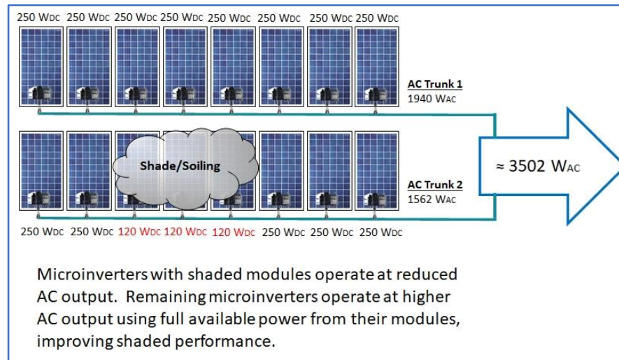
Figure 33: Microinverter – Shaded Operation - courtesy of Riverside Energy Systems with Microinverter Images Courtesy of Enphase
