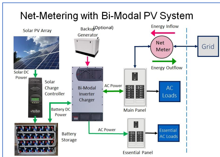
Figure 10: Net-Metering Solar PV system with Bi-Modal Inverter - courtesy of Riverside Energy Systems with equipment images courtesy of Outback Power Systems.
