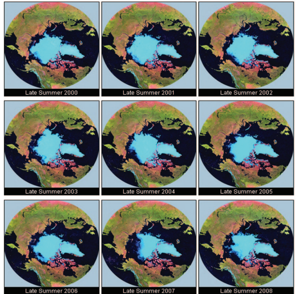
Circumpolar Arctic mapping from MODIS 250m spatial resolution, 9,000 km x 9,000 km
