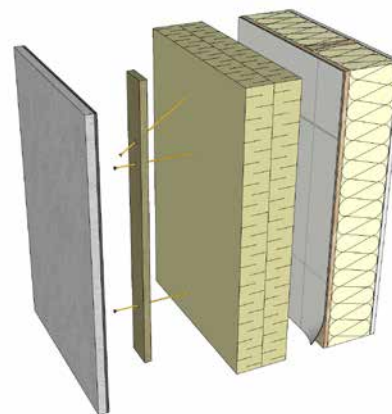
Figure 12 Screws installed at an upward angle can be used to limit deflection and support heavier-weight claddings if needed.
