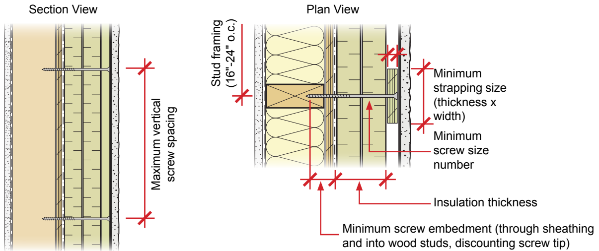
Figure 24 Design aspects of the strapping and fastener installation
