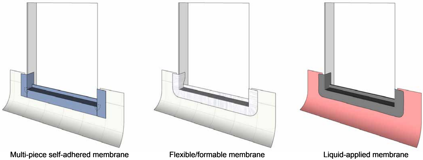
Figure 16 Examples of window sill membrane installation at the rough opening
