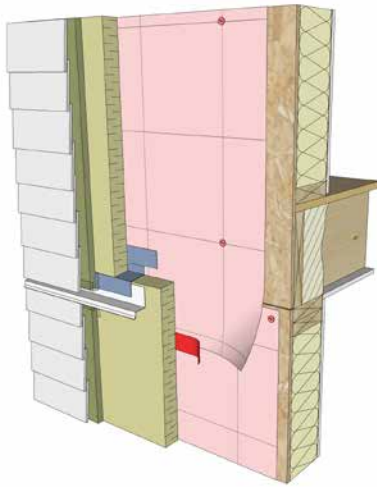
Figure 25 Mechanically fastened sealed sheathing membrane, with all edges of the airtight material taped.
