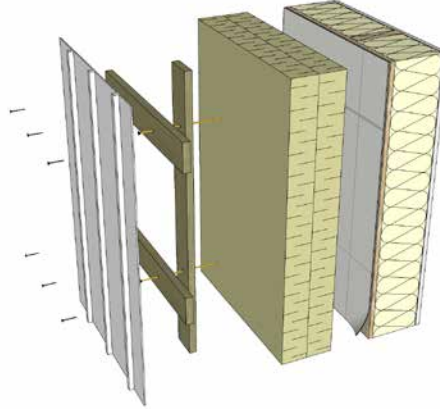
Figure 14 Cross-strapping is used to produce a horizontal strapping substrate for vertical cladding.
