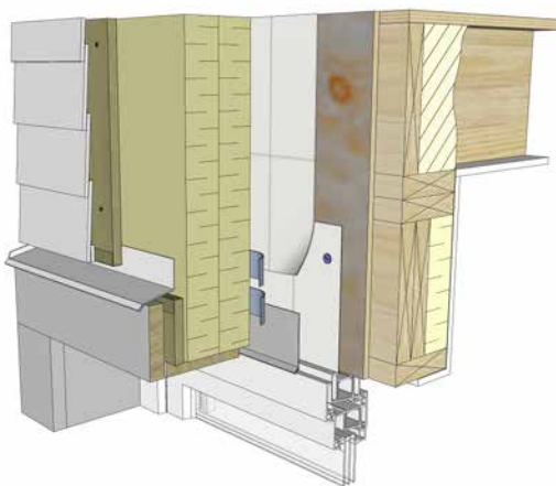
Figure 22 Window head flashing installed at the front face of the exterior insulation with secondary flashing installed directly above window.
