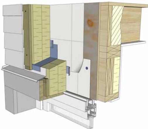
Figure 20 Window head flashing with taped through-wall flashing membrane.
