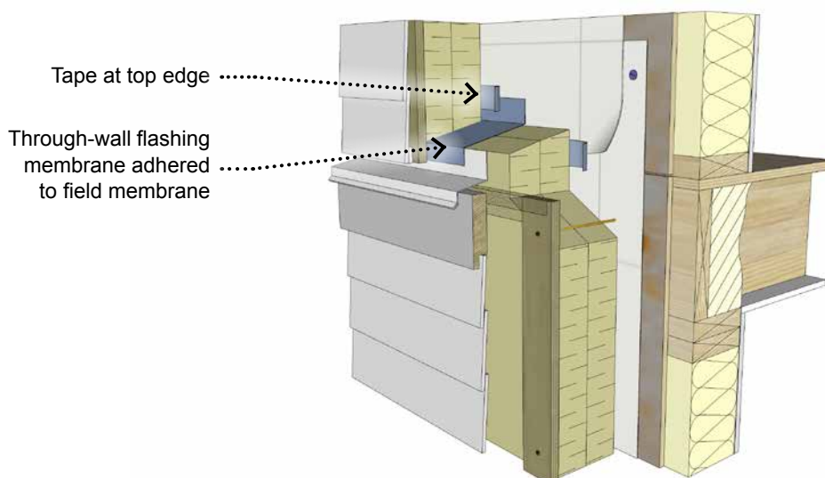
Figure 9 Simplified through-wall flashing approach (without positive laps)
