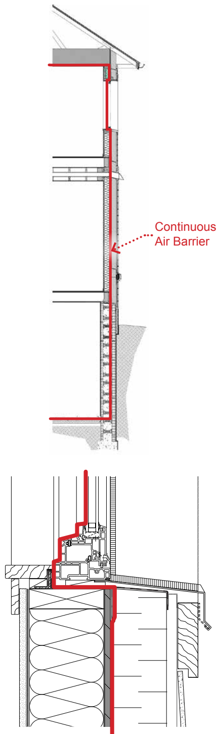
Figure 29 Example air barrier lines of continuity across the entire building enclosure and including all transition details.
