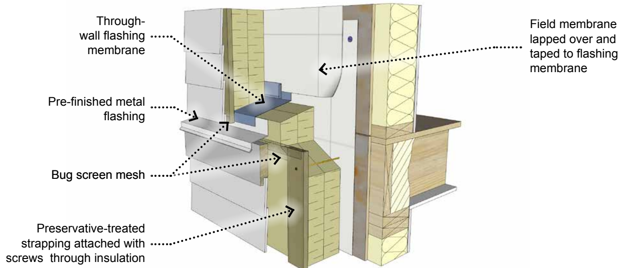
Figure 8 Conventional through-wall flashing detail and strapping installation
