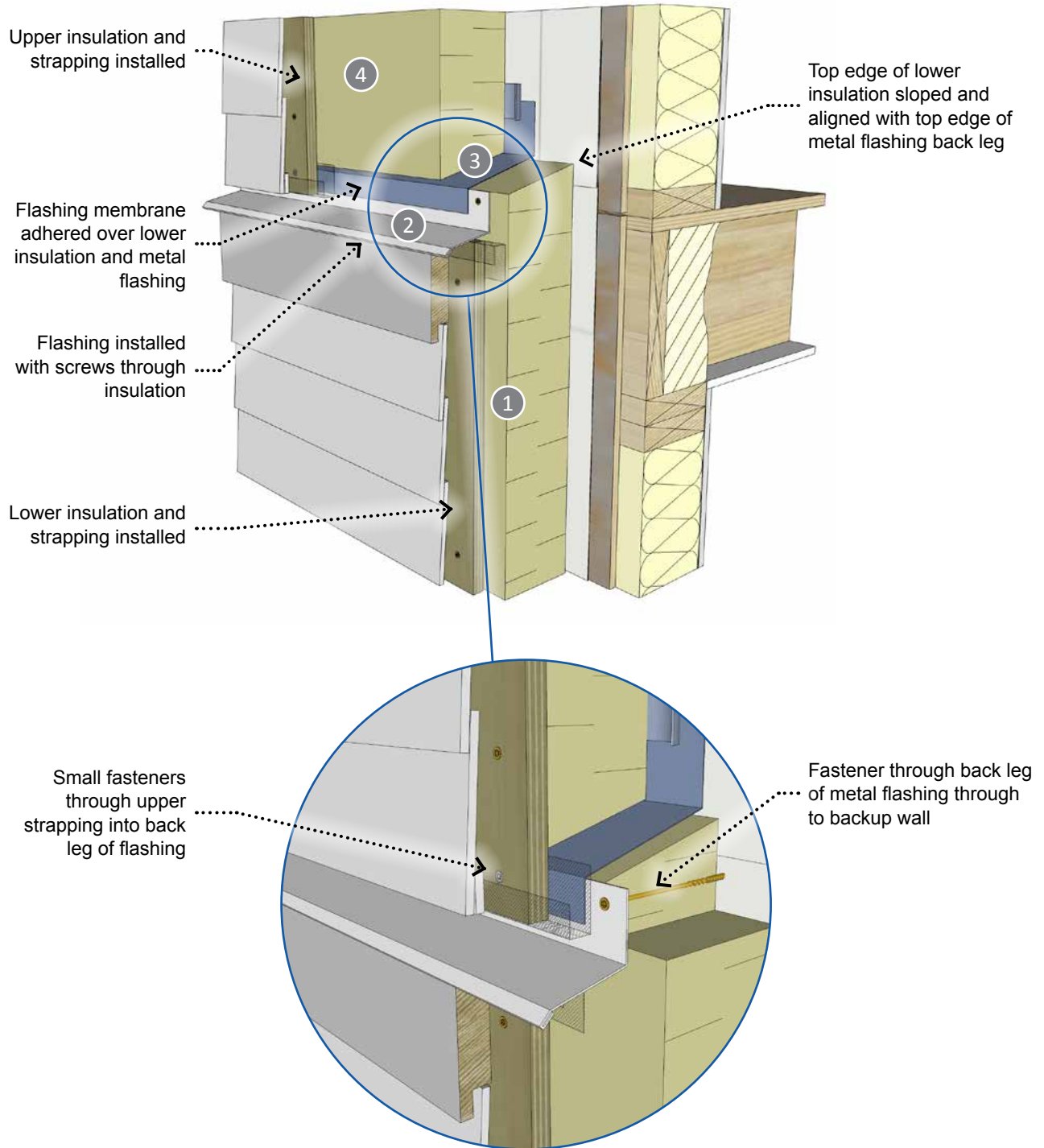
Figure 10 Through-wall flashing installation: metal flashing installed with screws at the front face of the exterior insulation, flashing membrane installed over lower insulation and adhered to metal flashing, and upper strapping used to secure flashing in place.
