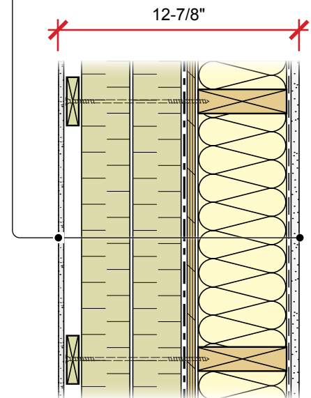
Figure 2 Typical assembly layers of the split-insulated wall with exterior vapour permeable rigid insulation
