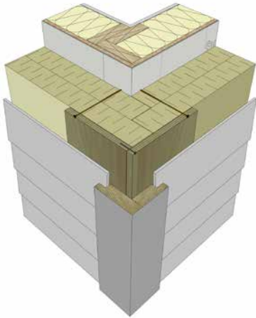
Figure 13 Wider corner strapping installation where corner trim must be installed onto strapping.
