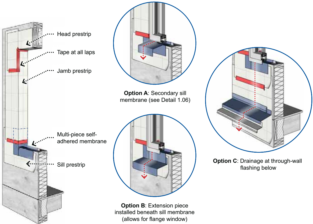
Figure 17 Window rough opening membrane installation at the sill, jamb and head.
