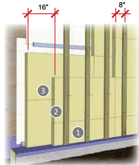
Figure 6 Exterior insulation installation method
