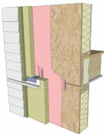
Figure 28 Liquid applied air barrier membrane
