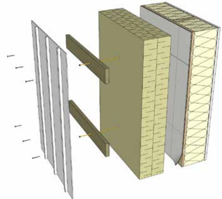
Figure 15 In dry climates with no rainscreen requirements, horizontal strapping alone can be used.
