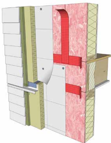
Figure 27 Sealed exterior sheathing air barrier approach
