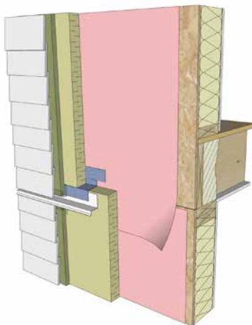
Figure 26 Vapour permeable self-adhered sheathing membrane, with all edges fully adhered to itself and the substrate to create an airtight layer.
