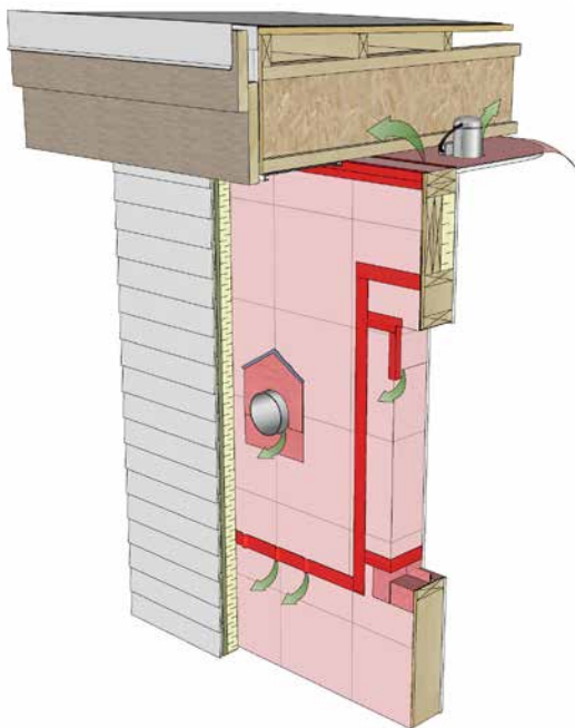
Figure 30 Common sheathing membrane and ceiling air barrier deficiencies.
