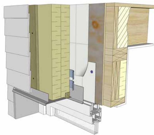
Figure 23 Window head flashing installed at the front face of the strapping with secondary flashing installed directly above window.
