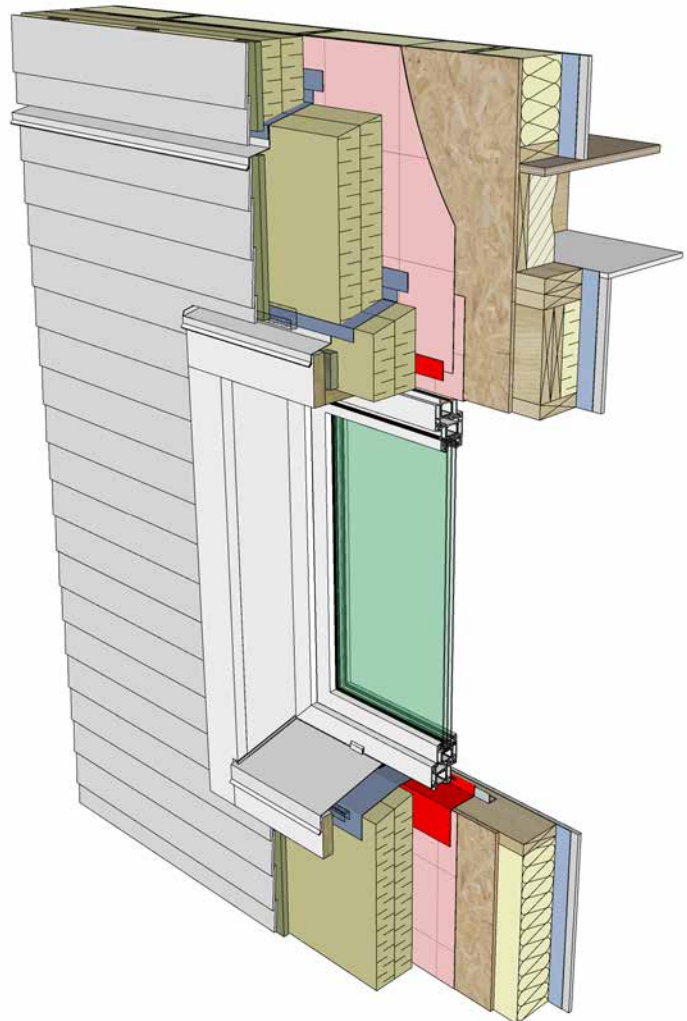
Figure 1 Split-insulated wall with exterior vapour permeable rigid insulation
