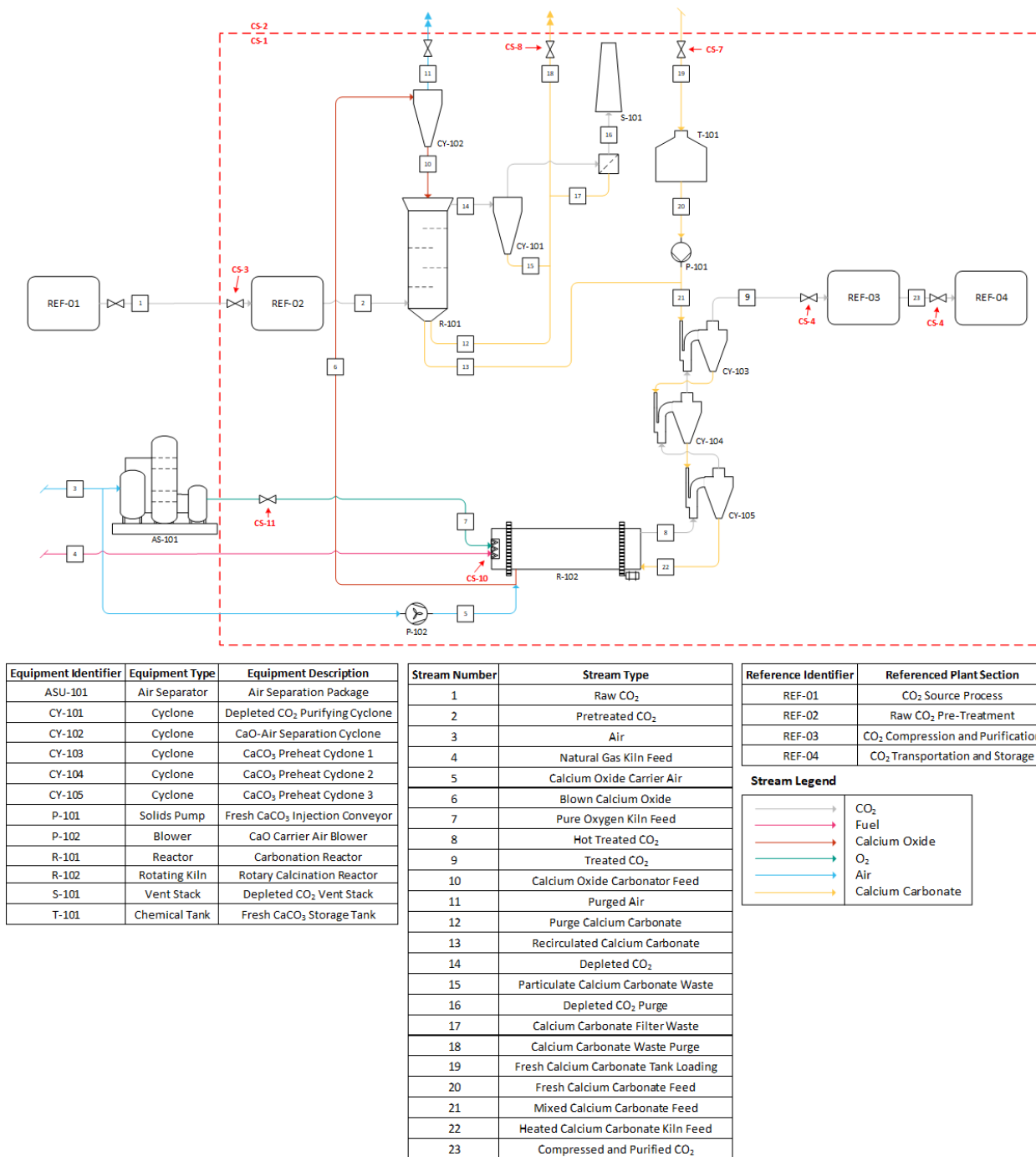
Figure 3.5-1: An example of a calcium looping carbon capture process.
