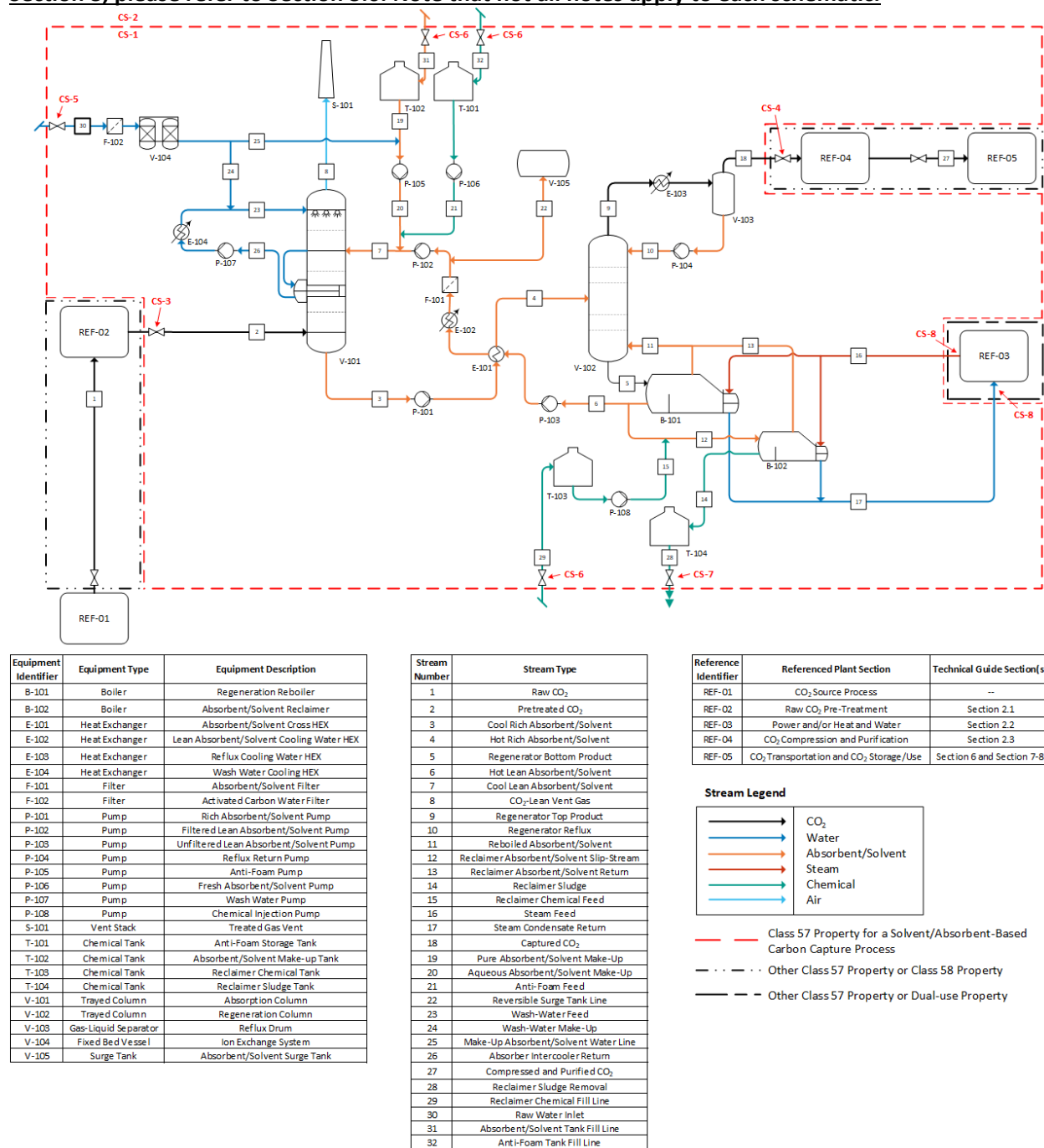
Figure 3.1-1: An example of an absorbent/solvent-based carbon capture process that uses an amine solvent.
