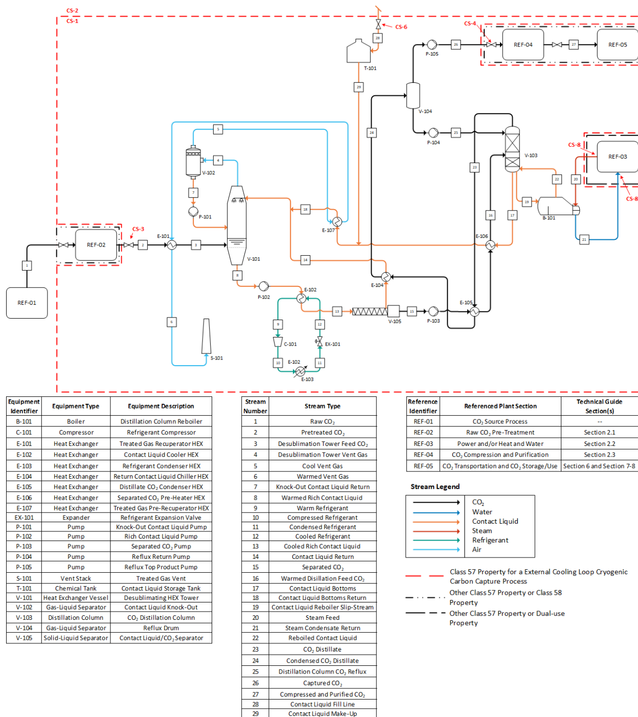
Figure 3.4-1: An example of external cooling loop cryogenic carbon capture process.
