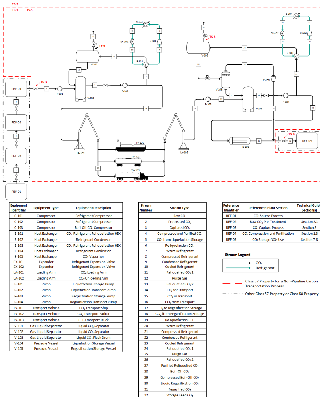
Figure 6.1-2: An example of a carbon transportation process using a transportation vehicle.
