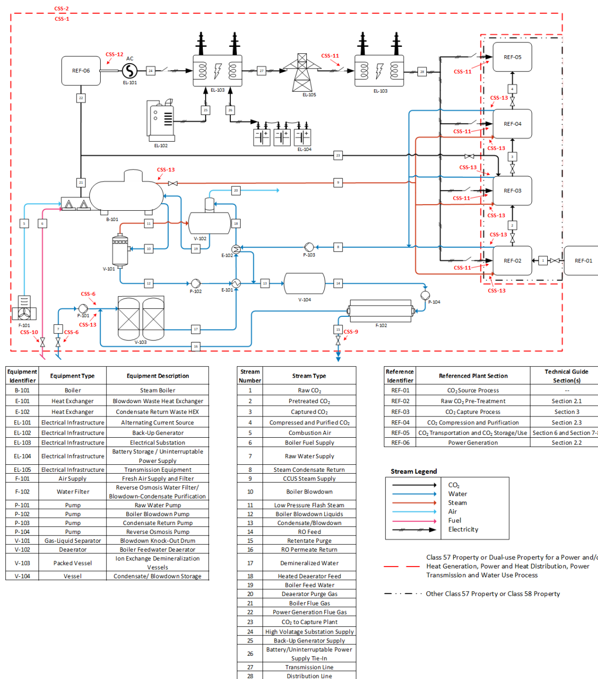
Figure 2.2-1: An example of a power and heat generation, power and heat distribution, power transmission, and water use process supporting a CCUS process.
