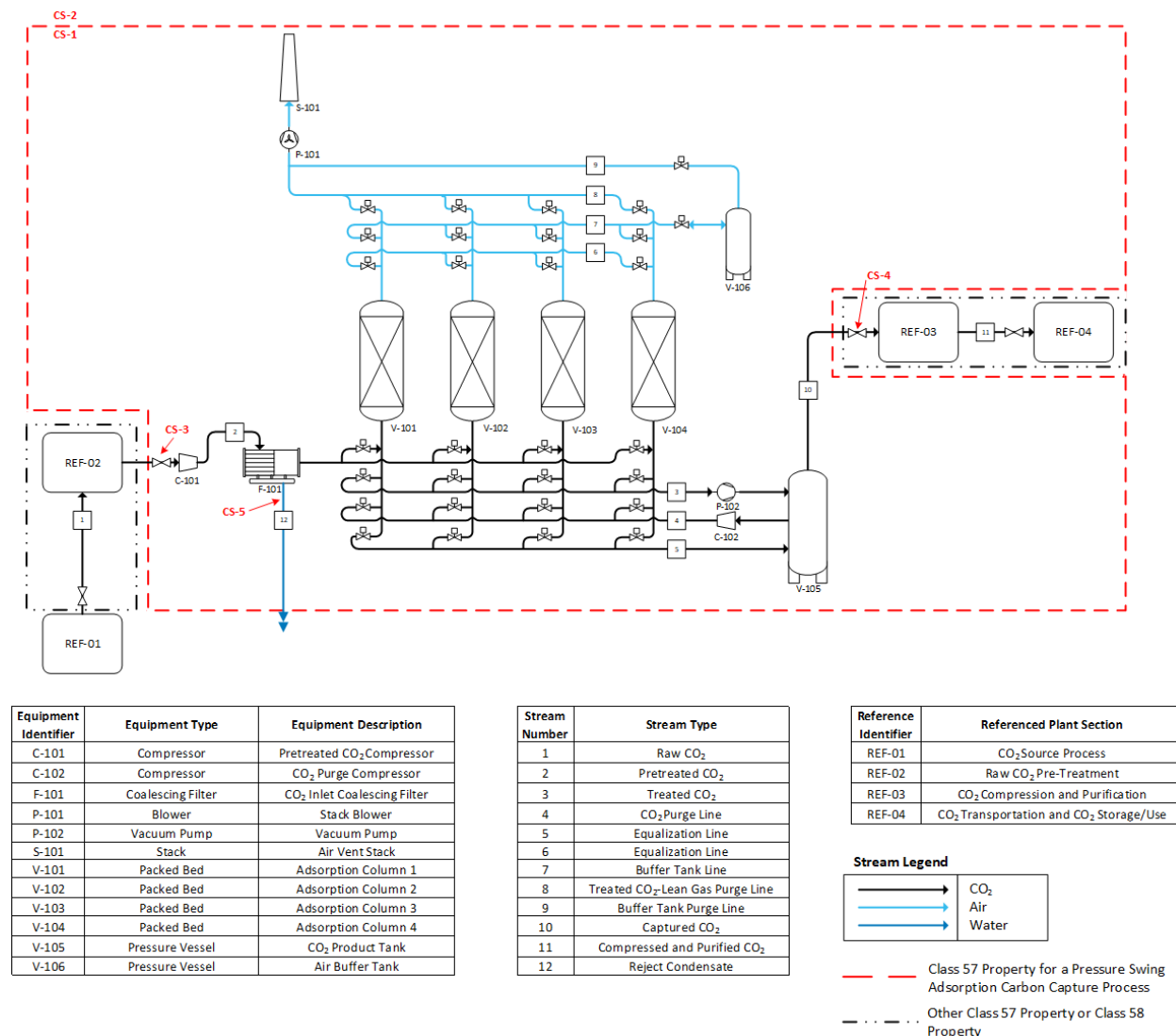
Figure 3.2-1: An example of a solid adsorption carbon capture process that uses pressure swing adsorption.
