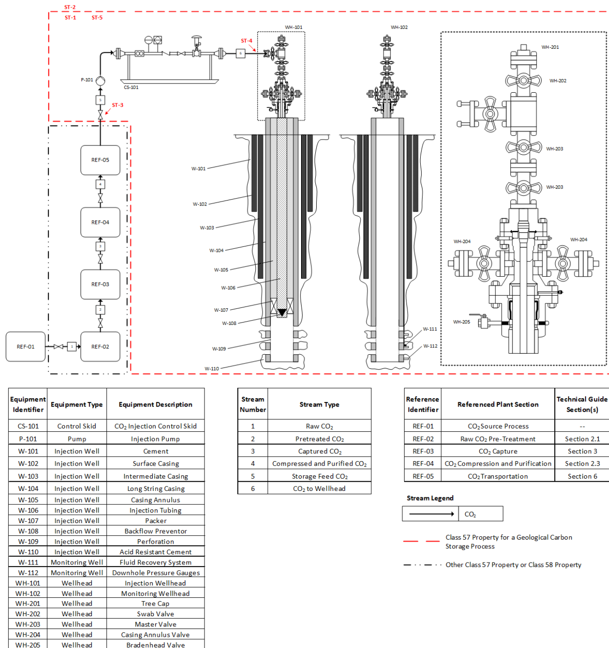
Figure 7.1-1: An example of an injection system for carbon storage in a geological formation.
