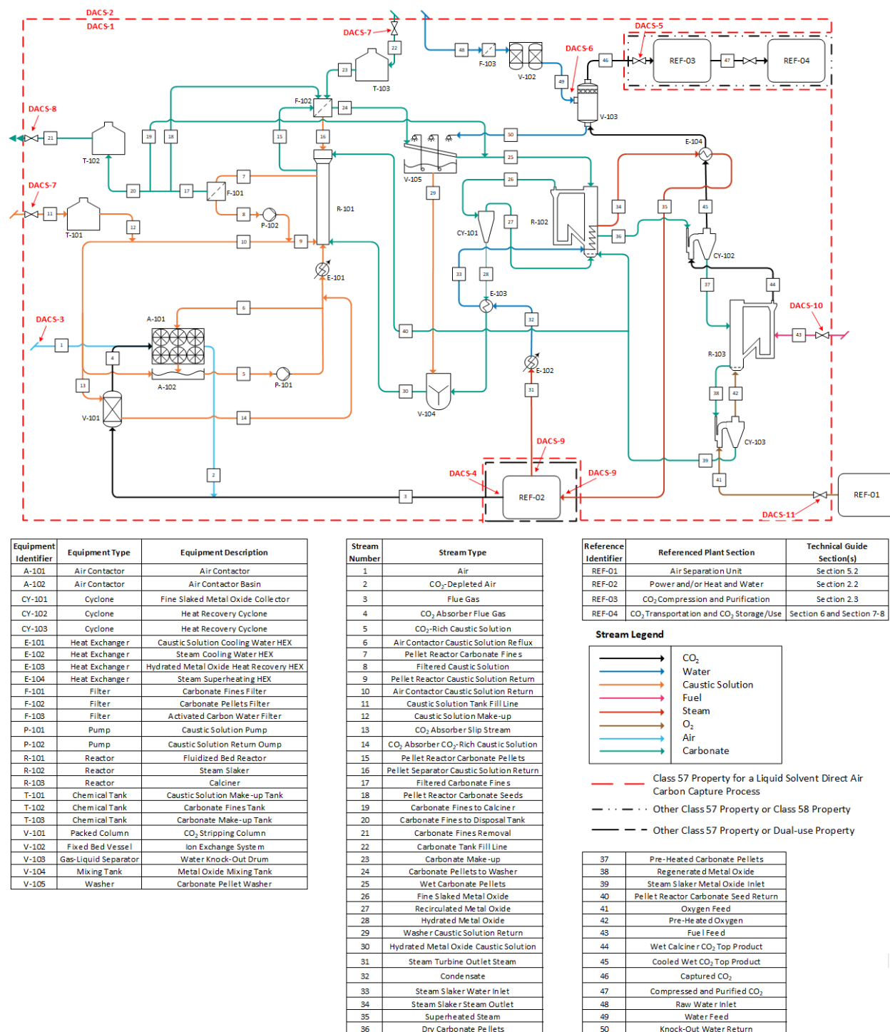
Figure 4.1-1: An example of a liquid solvent direct air capture process.
