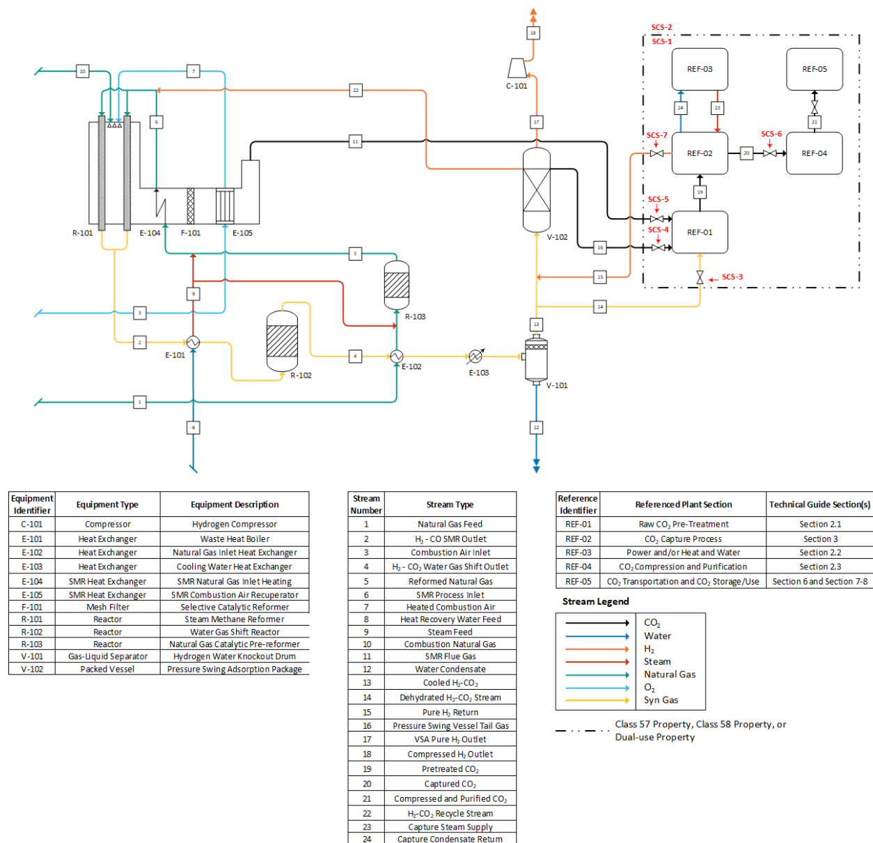
Figure 5.1-1: An example of carbon capture from SMR hydrogen production.
