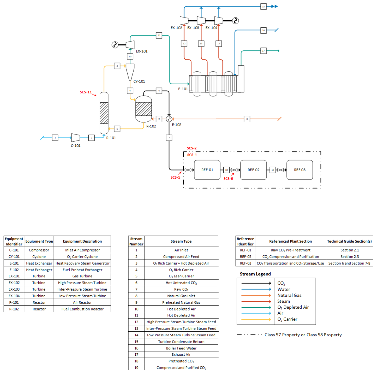
Figure 5.4-1: An example of carbon capture from a chemical looping process.
