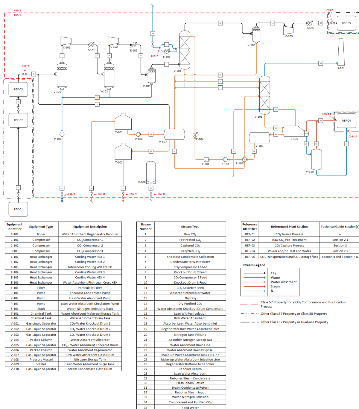
Figure 2.3-1: An example of a CO 2 purification and compression process with multi-stage compression and triethylene glycol dehydration.
