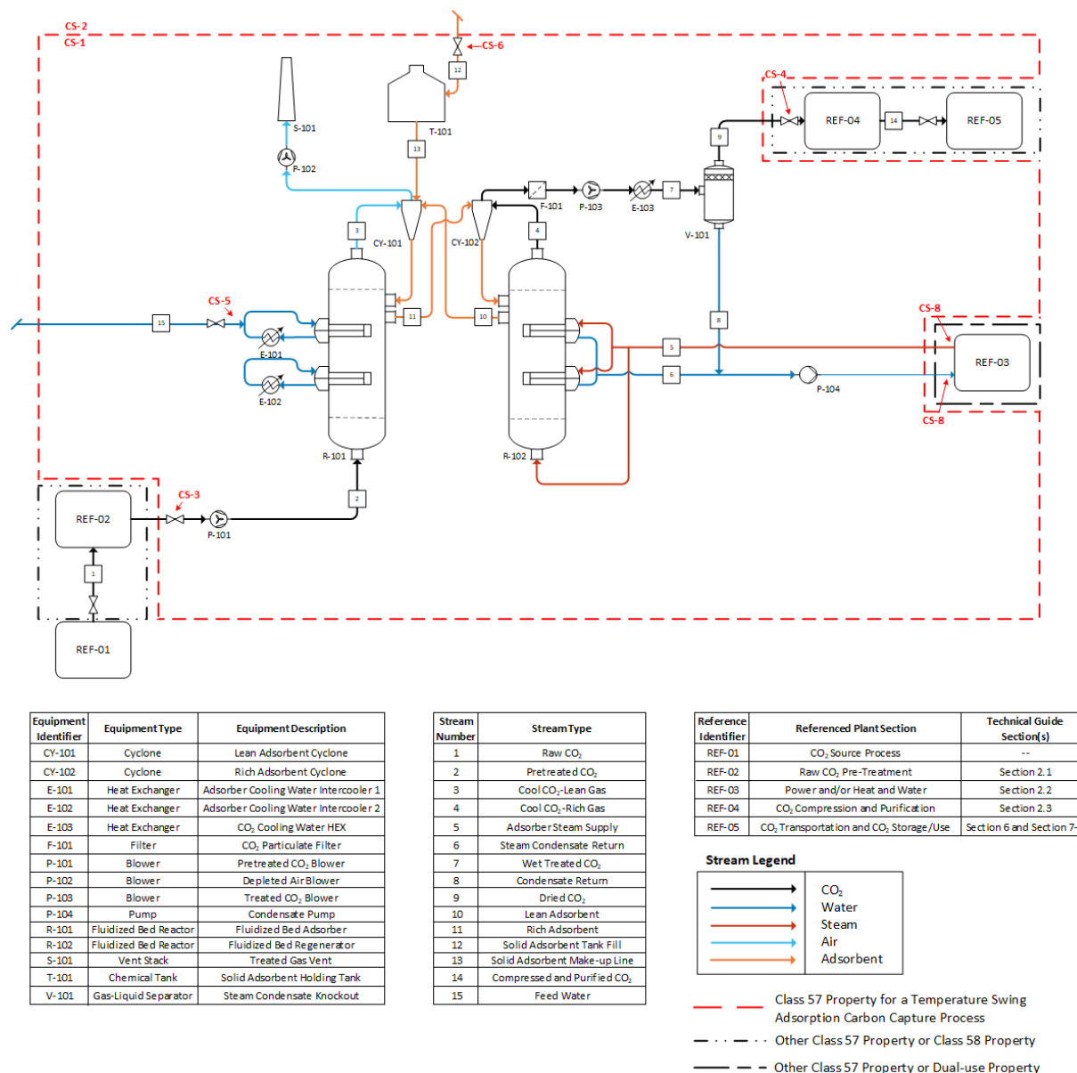
Figure 3.2-2: An example of a solid adsorption carbon capture process that uses temperature swing adsorption.
