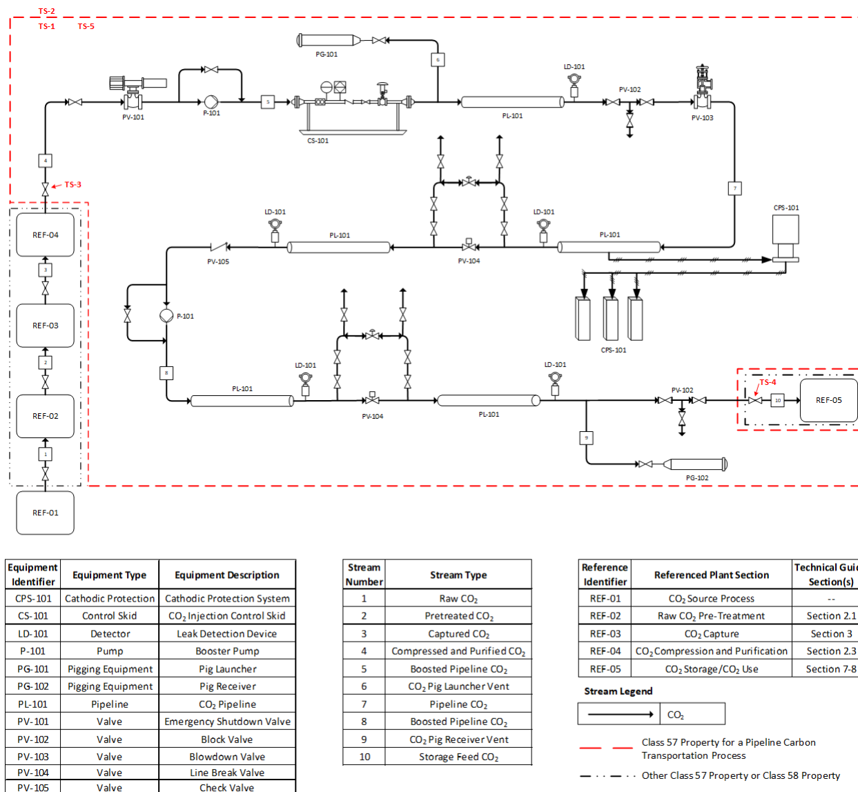
Figure 6.1-1: An example of a carbon transportation process using a pipeline.
